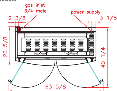
FB1400-4G on (heated) base cabinet
