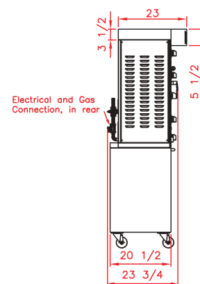
SIDE VIEW FB1400-4G shown
