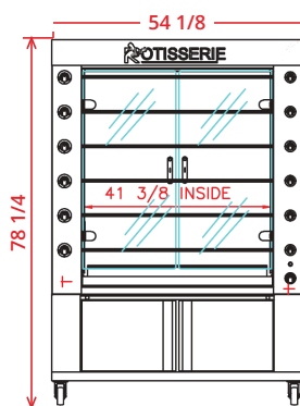
FB1400-6G on (heated) base cabinet
