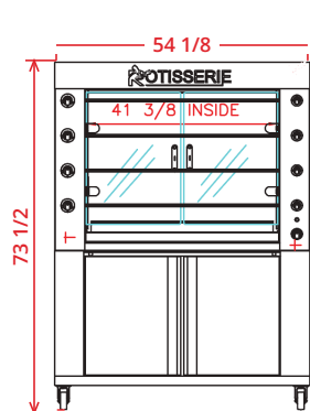
FB1400-4G on (heated) base cabinet
