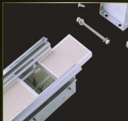
Removable and interchangeable ceramic inserts ( significant cost savings ).
