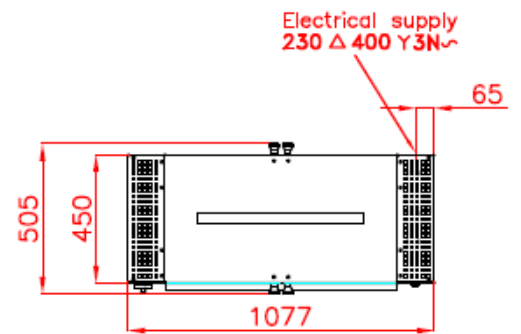
Top view Rotisserie and wheeled stand
