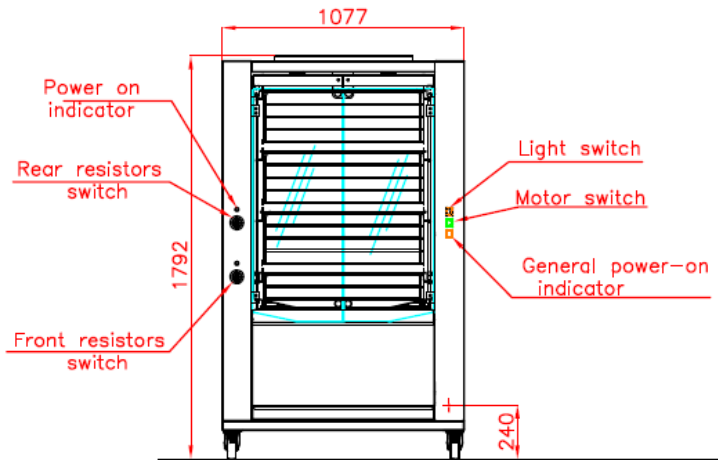
Front view Rotisserie and wheeled stand
