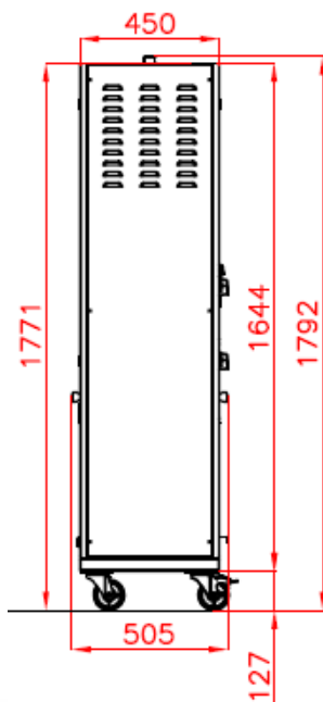
Side view Rotisserie and wheeled stand
